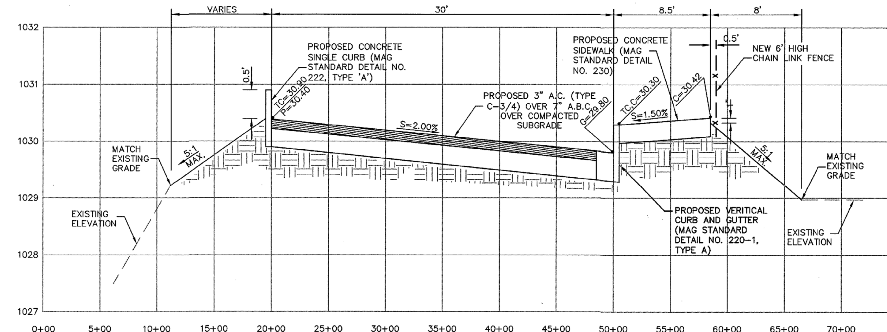
SECTION B-B HORIZONTAL: 1"=5' VERTICAL: 1"=1'
