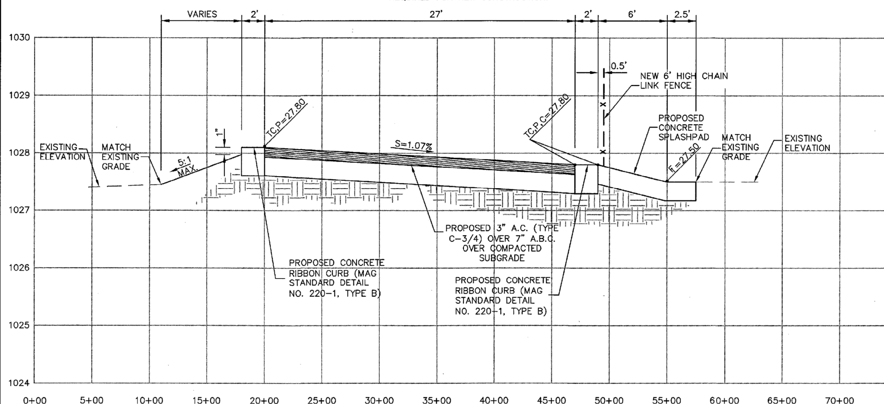
SECTION A-A HORIZONTAL: 1"=5' VERTICAL: 1"=1'
